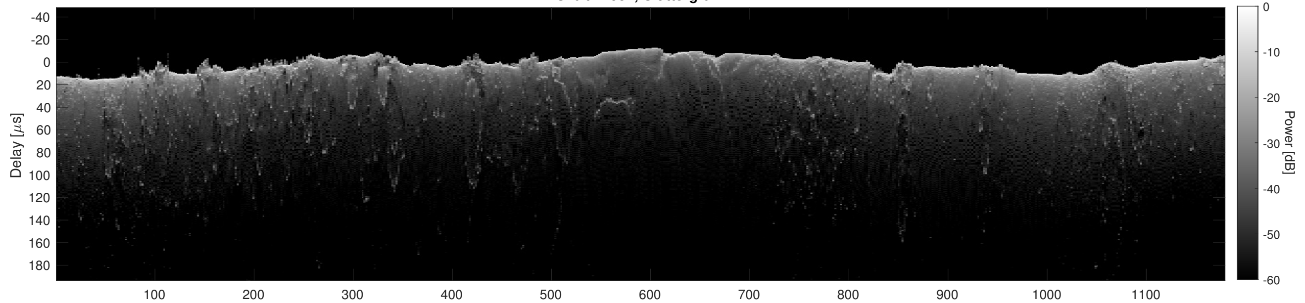
Orbit 12952, Cluttergram
