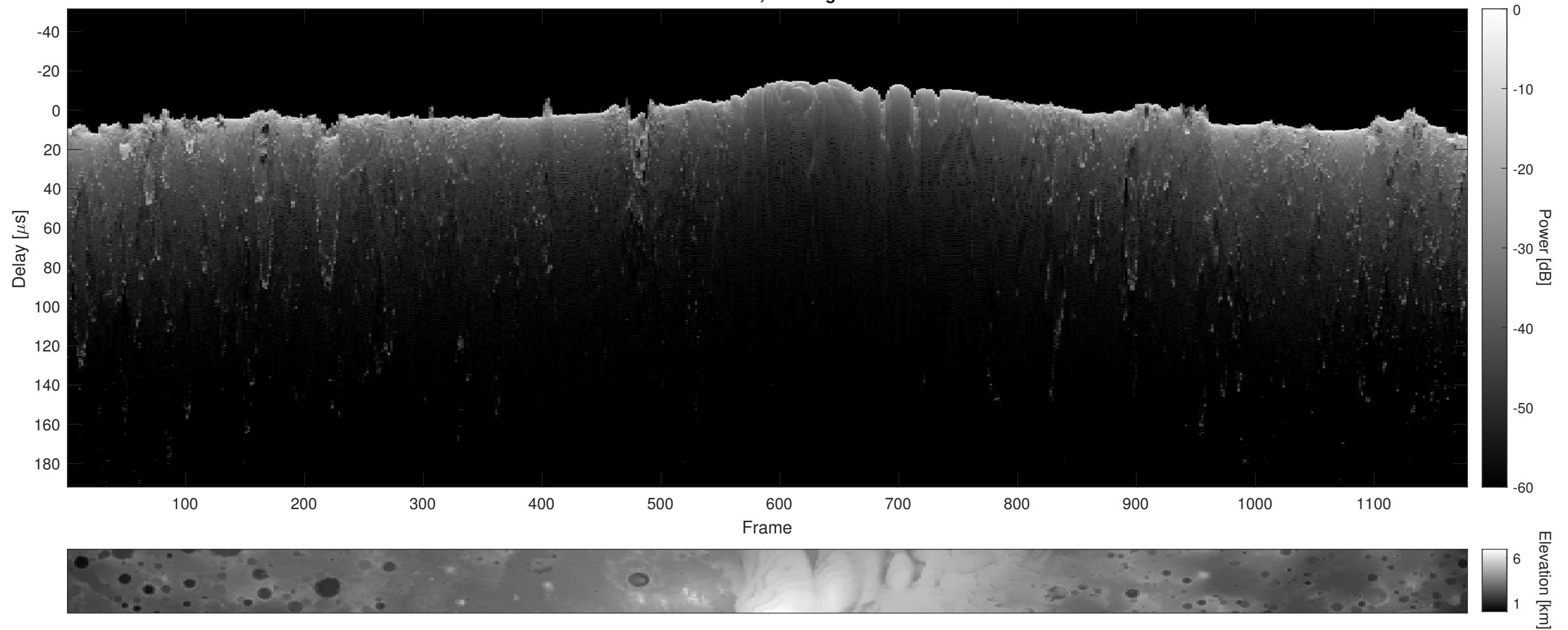
Orbit 12953, Cluttergram
