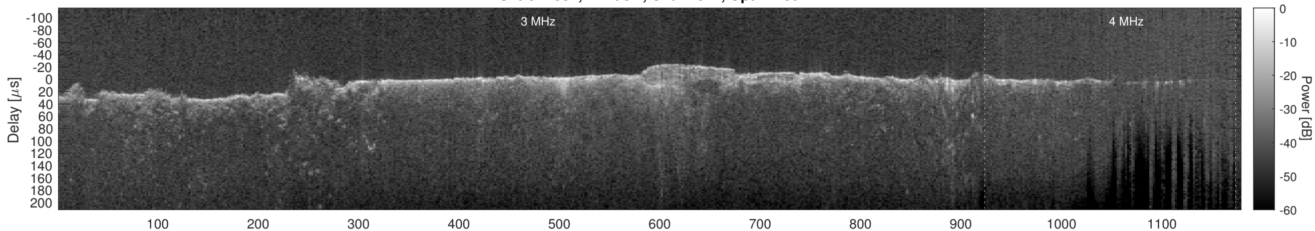
Orbit 12957, Cluttergram
