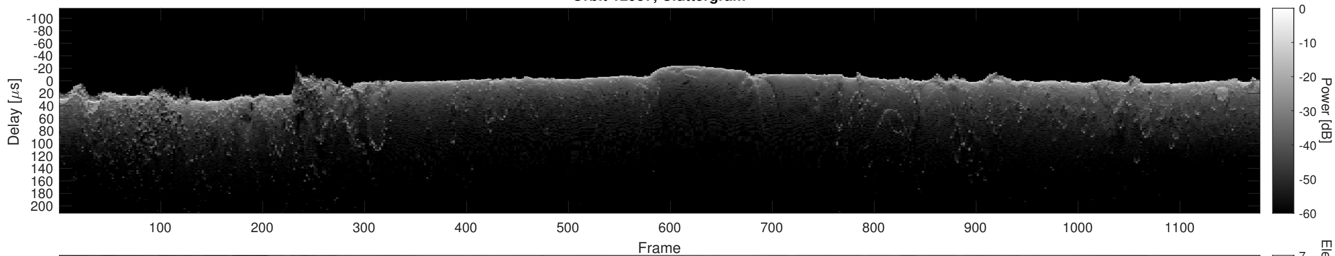
Orbit 12957, Cluttergram
