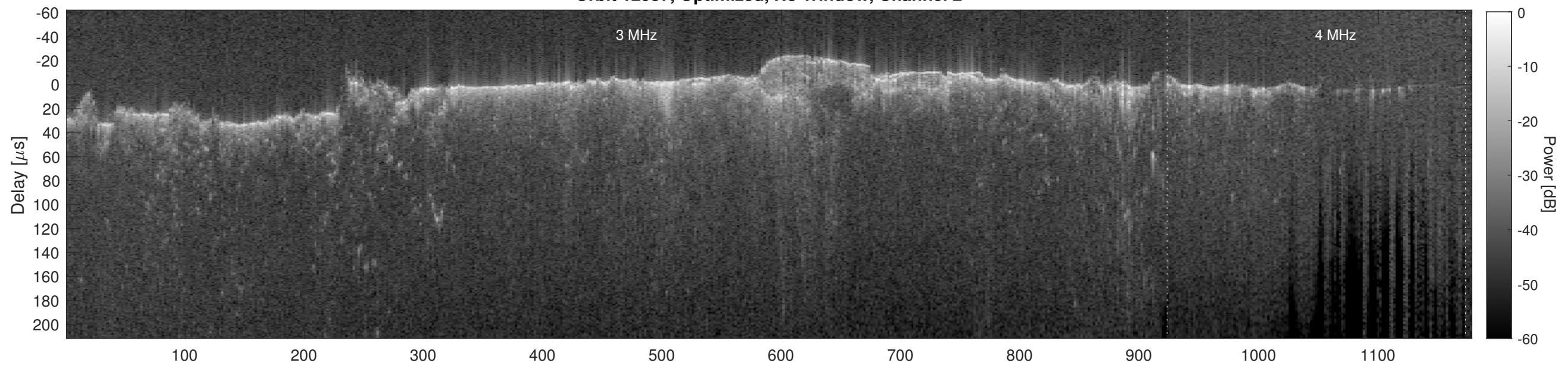
Orbit 12957, Cluttergram
