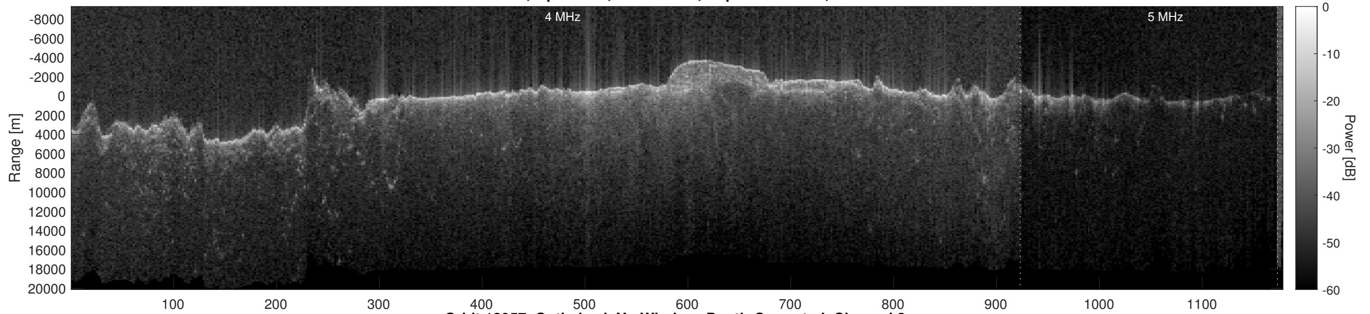
Orbit 12957, Optimized, No Window, Depth-Corrected, Channel 2
