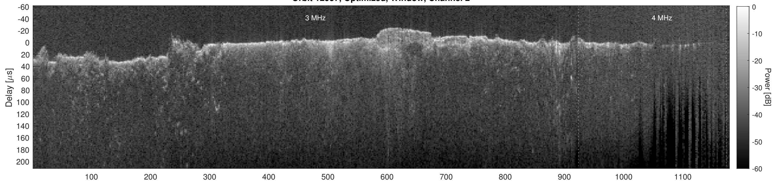
Orbit 12957, Cluttergram
