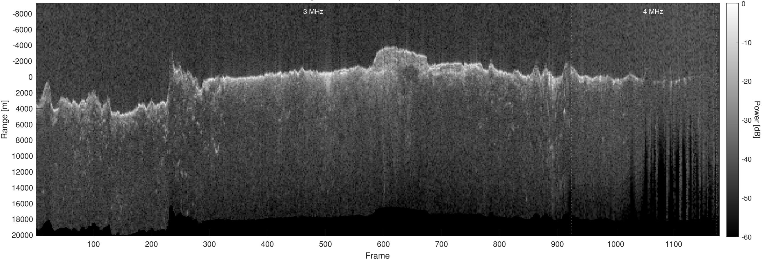
Orbit 12957, Optimized, Window, Depth-Corrected, Channel 2
