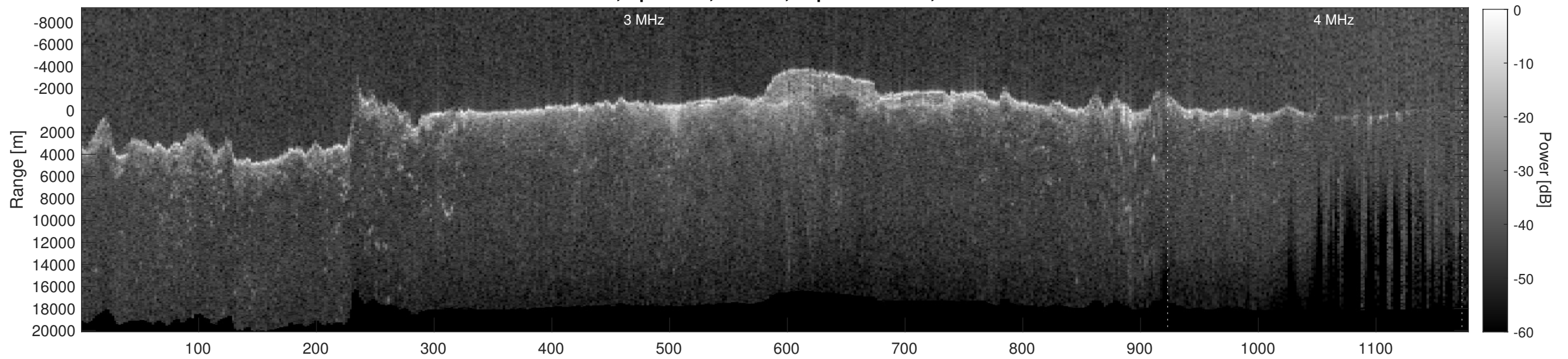
Orbit 12957, Depth-Corrected Cluttergram
