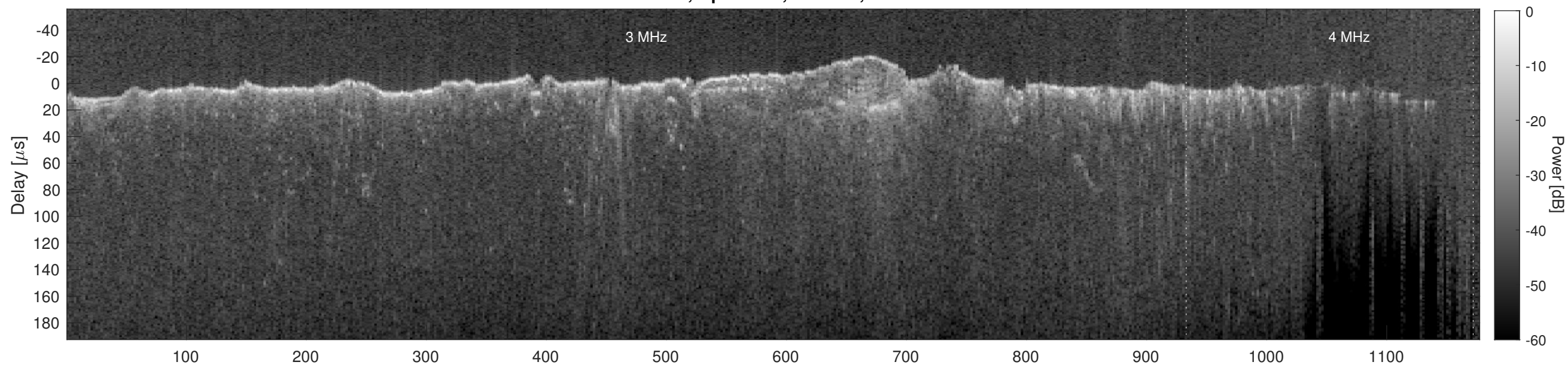
Orbit 12958, Cluttergram
