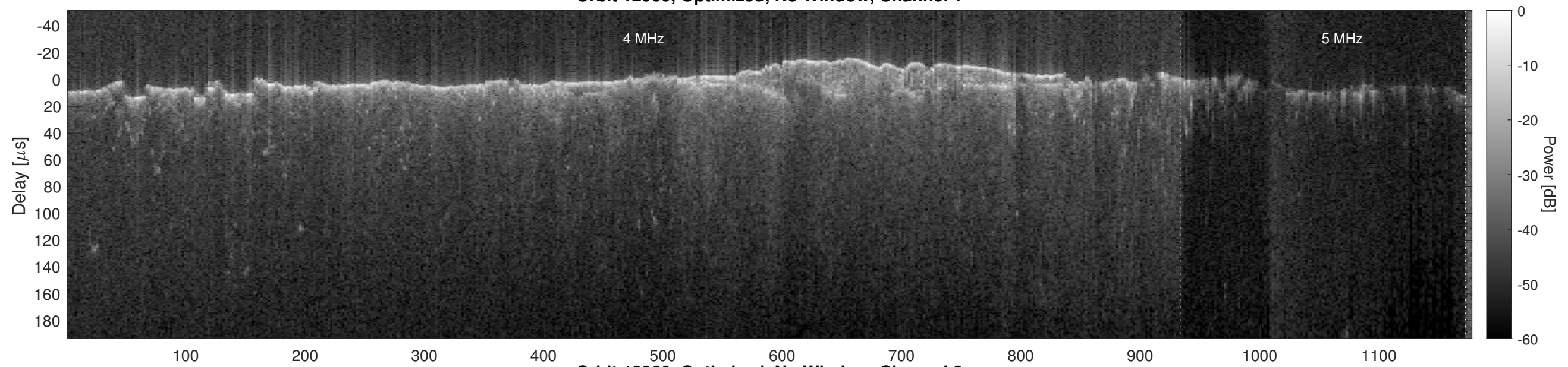
Orbit 12960, Optimized, No Window, Channel 2
