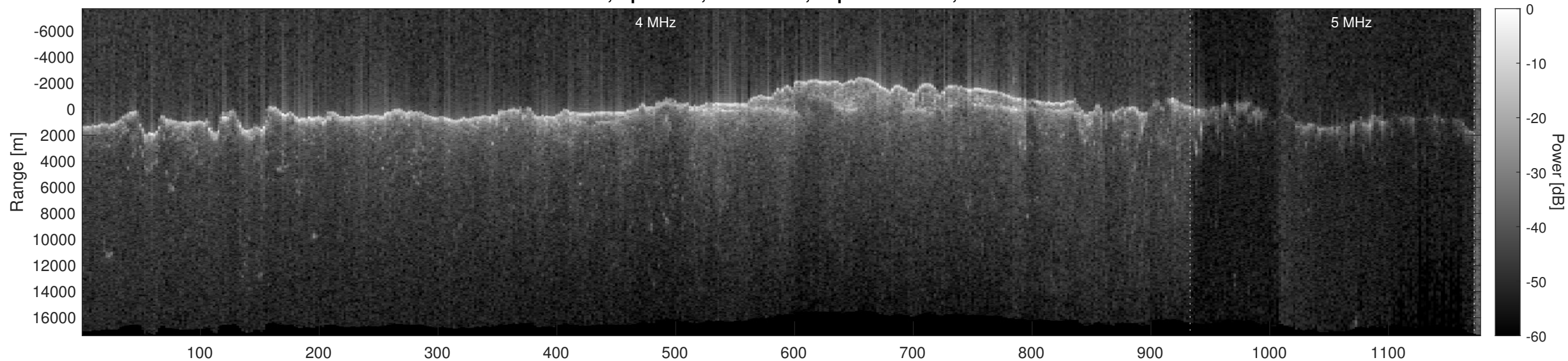
Orbit 12960, Optimized, No Window, Depth-Corrected, Channel 2
