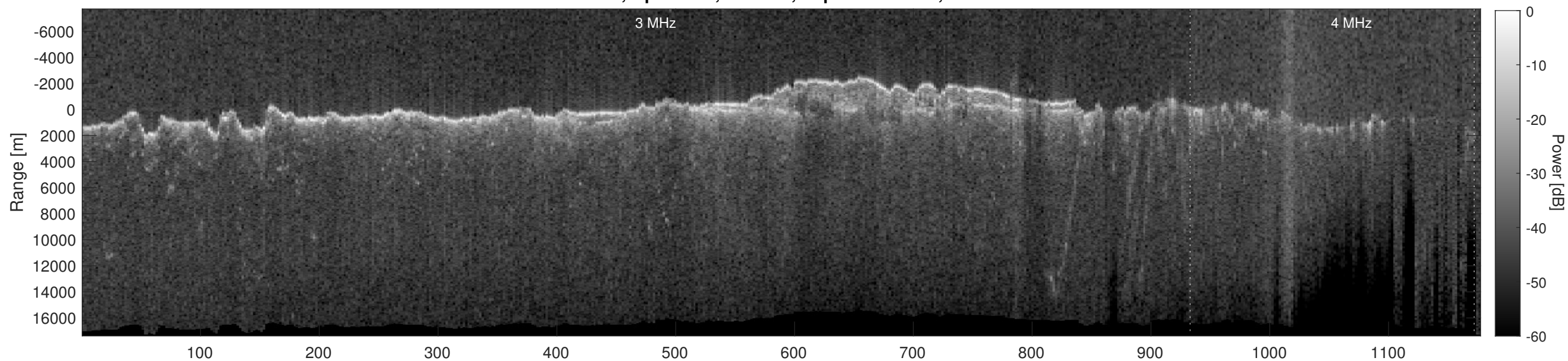
Orbit 12960, Depth-Corrected Cluttergram
