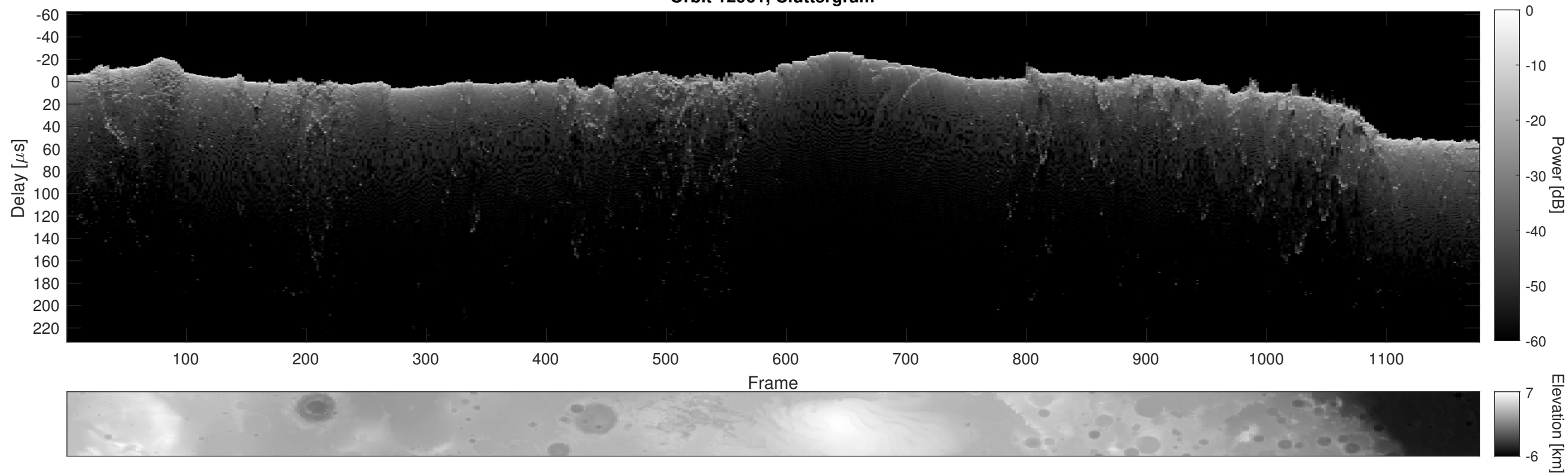
Orbit 12961, Cluttergram
