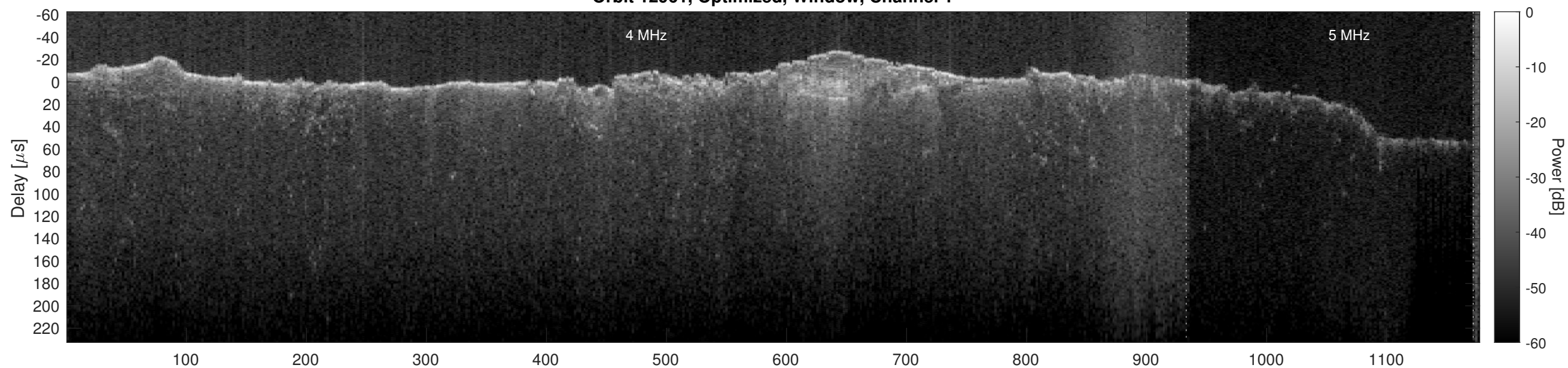
Orbit 12961, Optimized, Window, Channel 2
