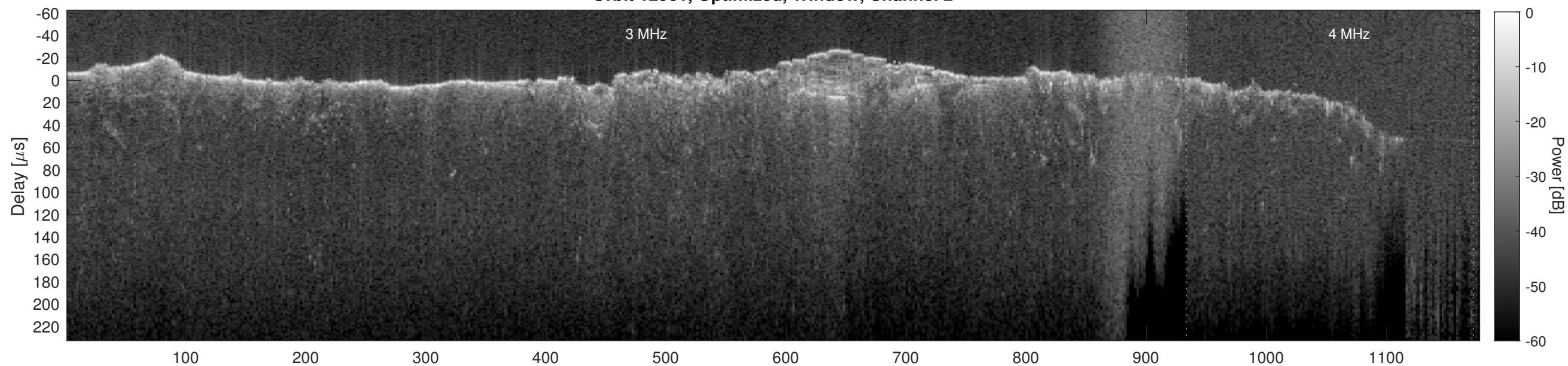
Orbit 12961, Cluttergram
