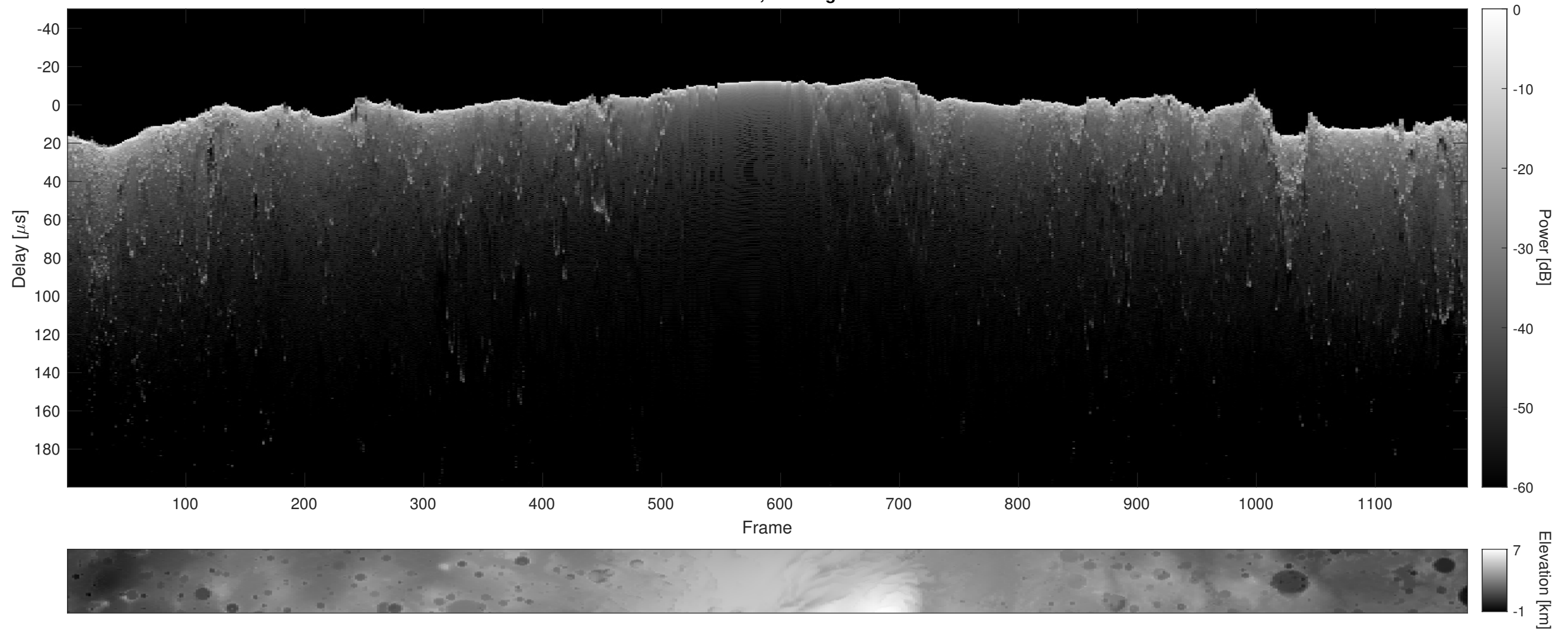
Orbit 12962, Cluttergram
