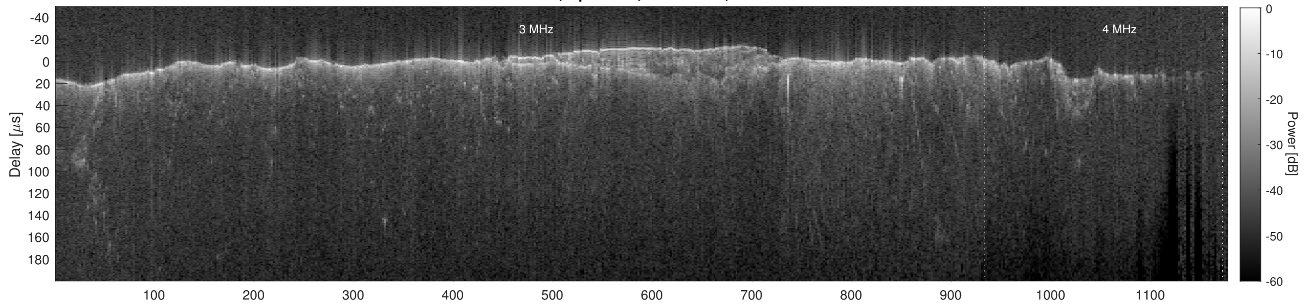
Orbit 12962, Cluttergram
