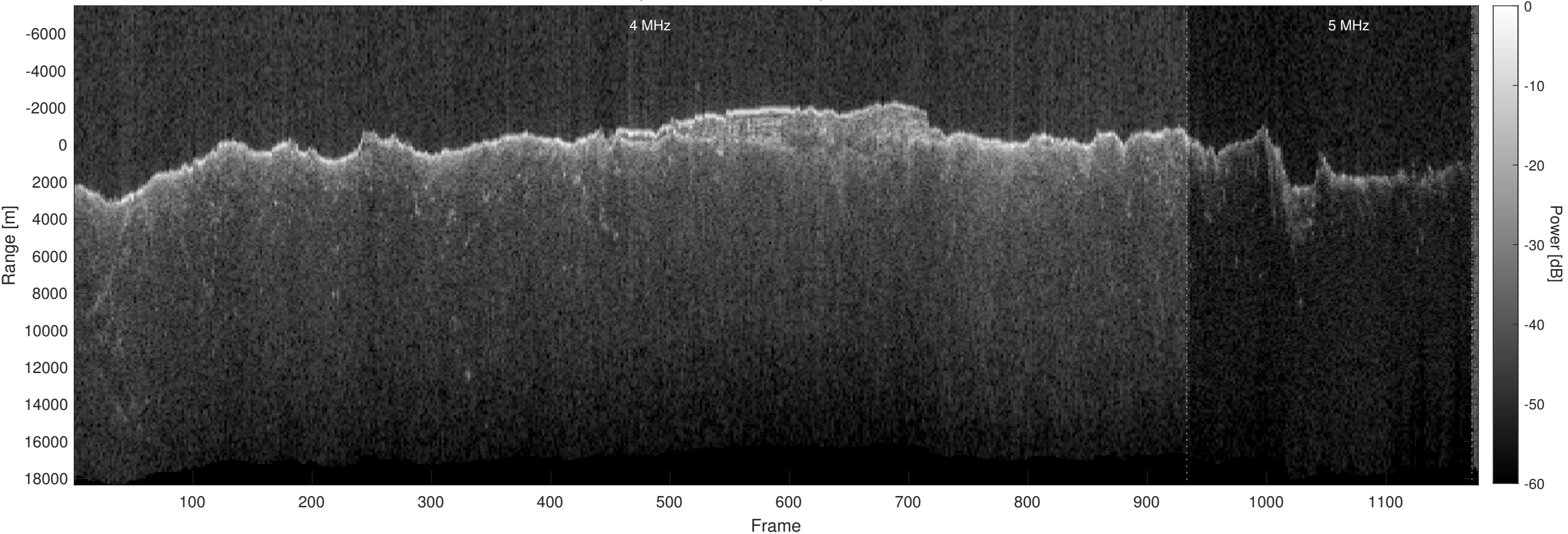
Orbit 12962, Optimized, Window, Depth-Corrected, Channel 2
