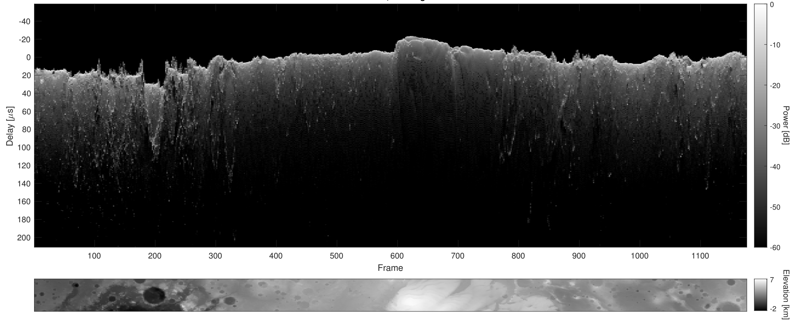
Orbit 12964, Cluttergram
