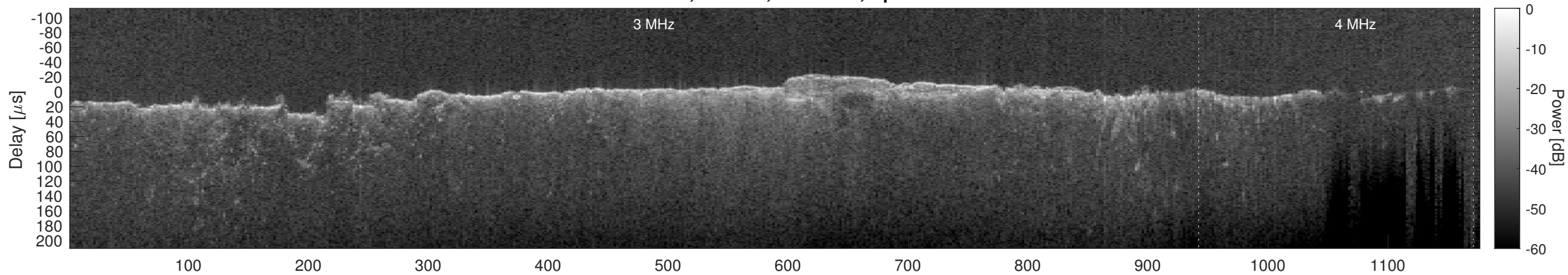
Orbit 12964, Cluttergram
