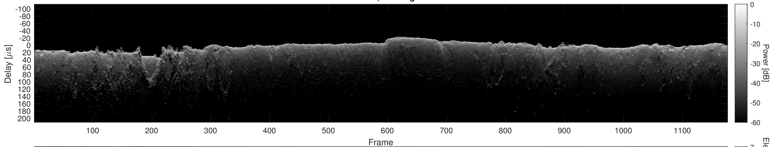
Orbit 12964, Cluttergram
