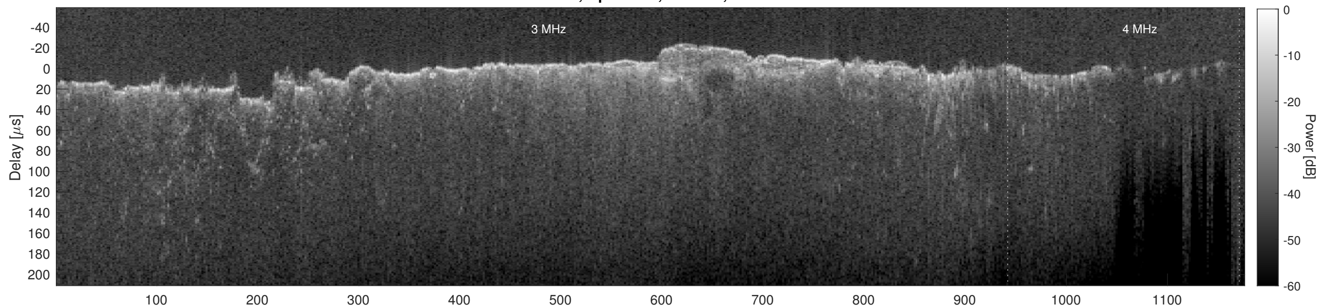
Orbit 12964, Cluttergram
