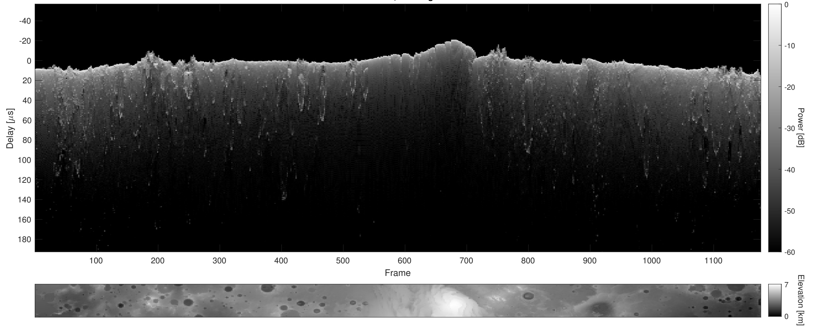
Orbit 12965, Cluttergram
