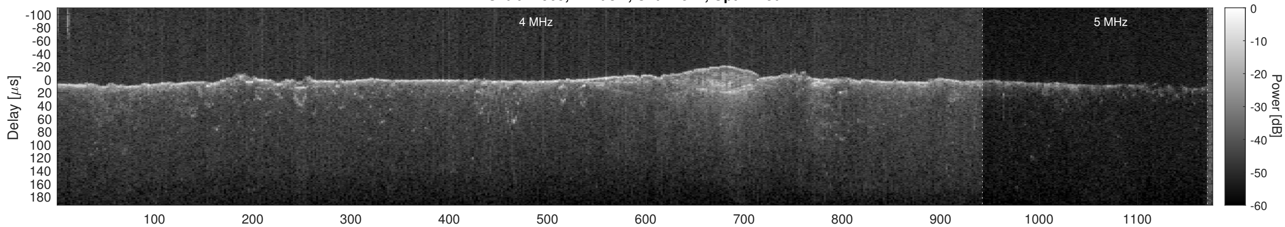
Orbit 12965, Cluttergram
