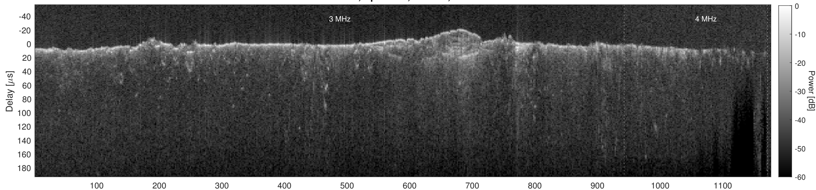
Orbit 12965, Cluttergram
