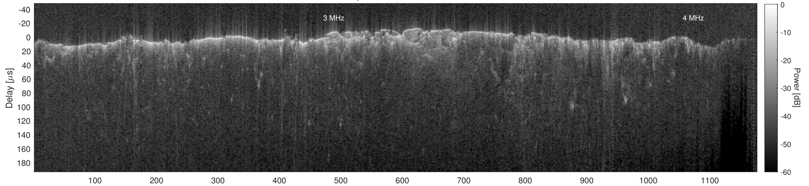
Orbit 12966, Cluttergram
