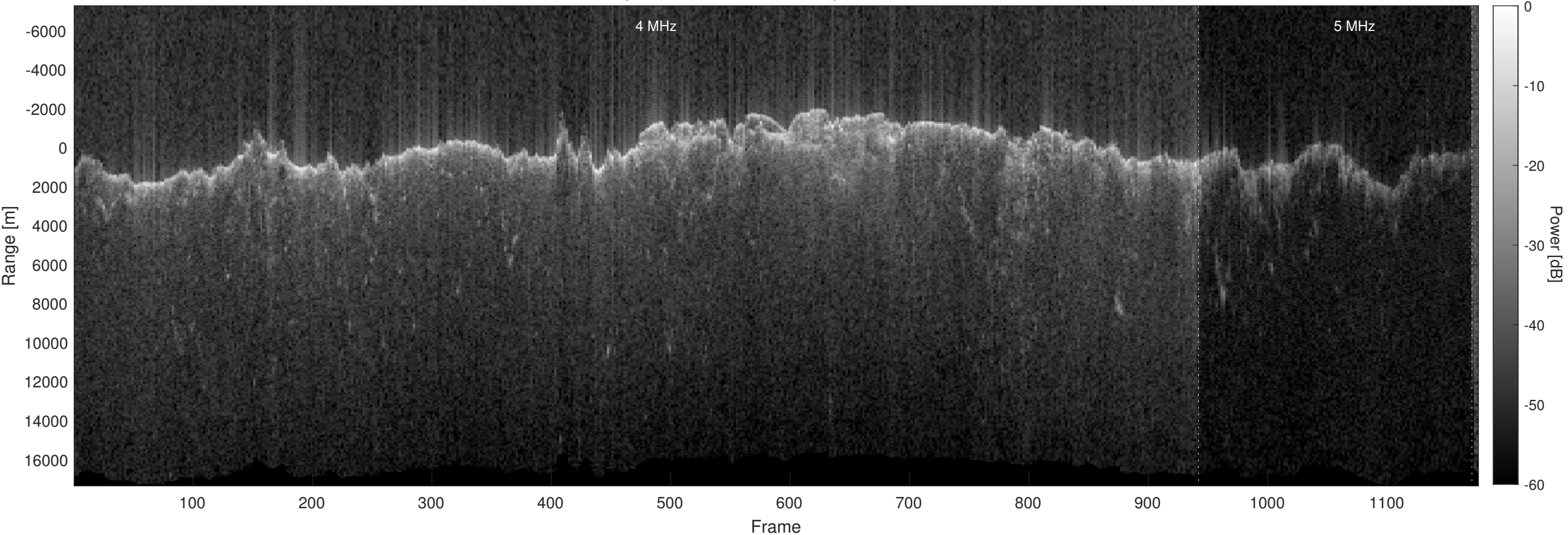
Orbit 12966, Optimized, No Window, Depth-Corrected, Channel 2
