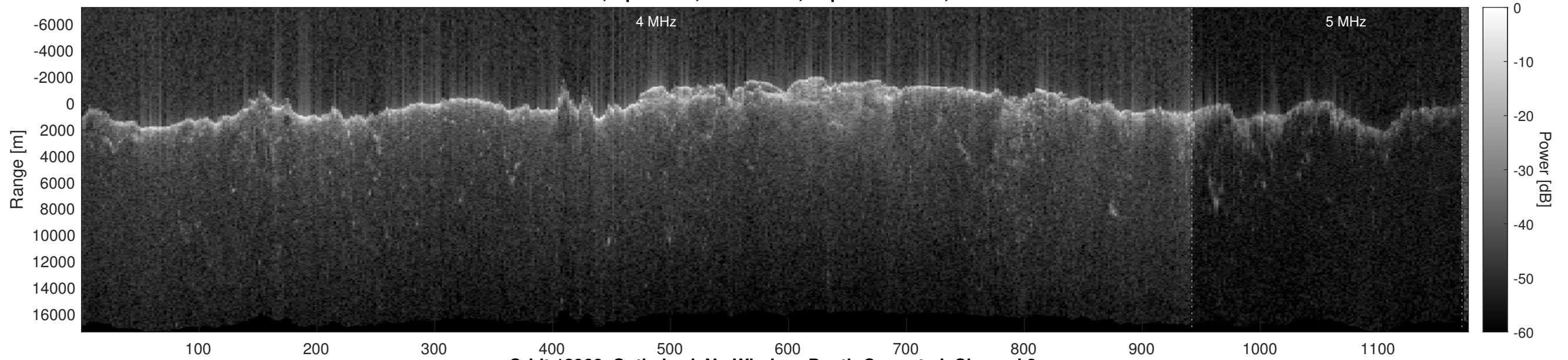
Orbit 12966, Optimized, No Window, Depth-Corrected, Channel 2
