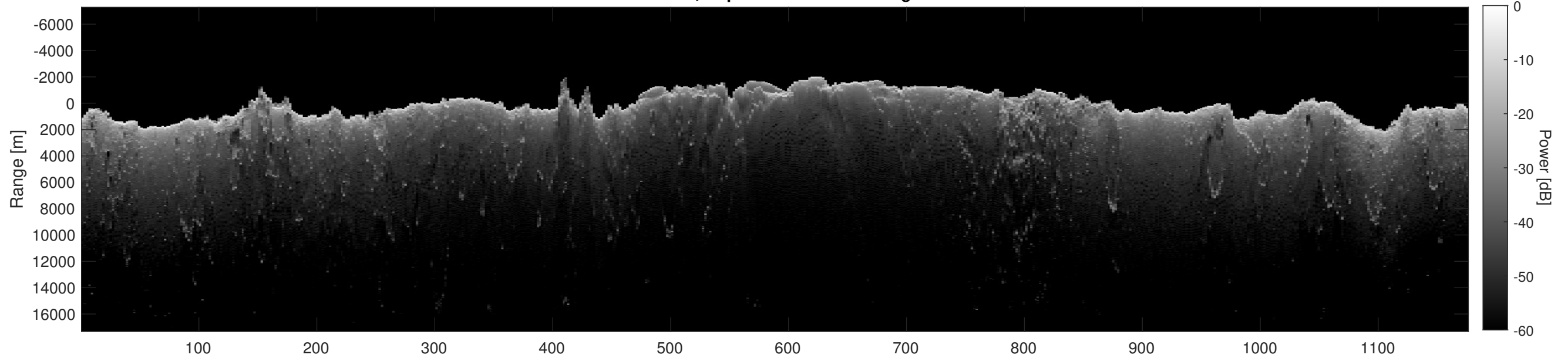
Orbit 12966, Depth-Corrected Cluttergram
