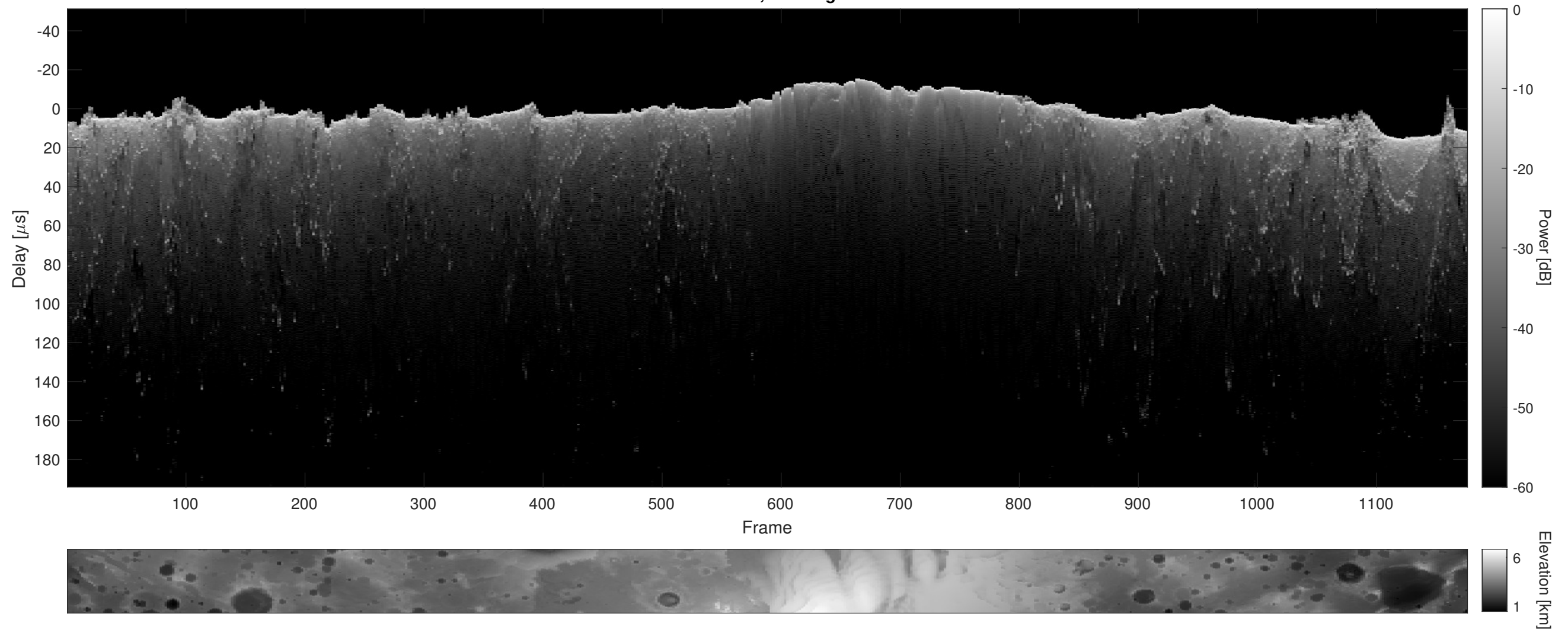
Orbit 12967, Cluttergram
