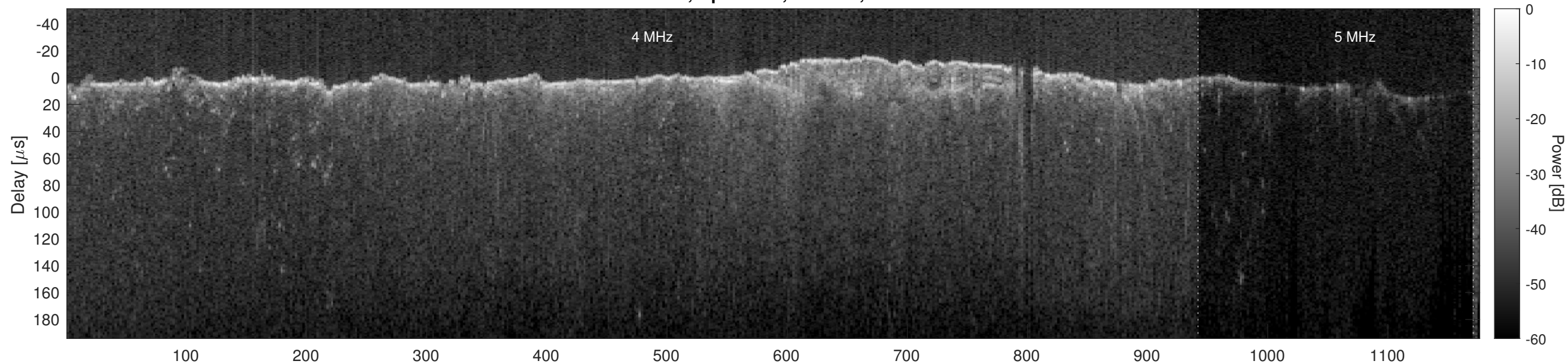
Orbit 12967, Optimized, Window, Channel 2
