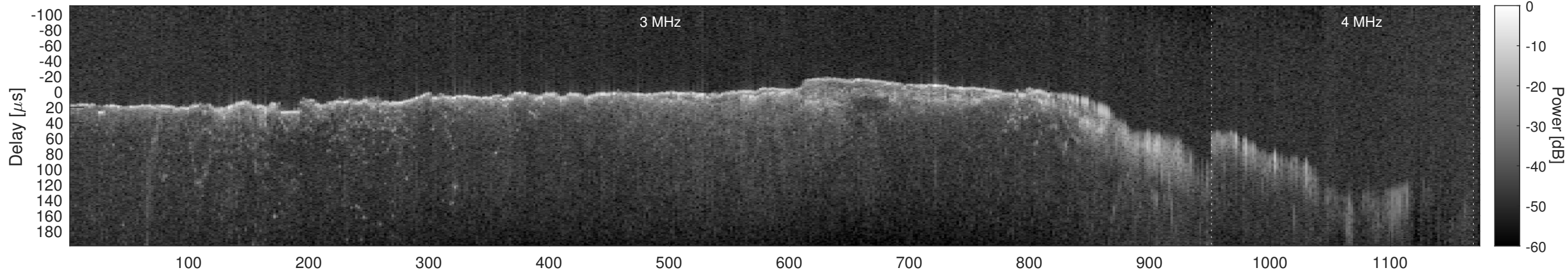
Orbit 12971, Window, Channel 2, Chapman
