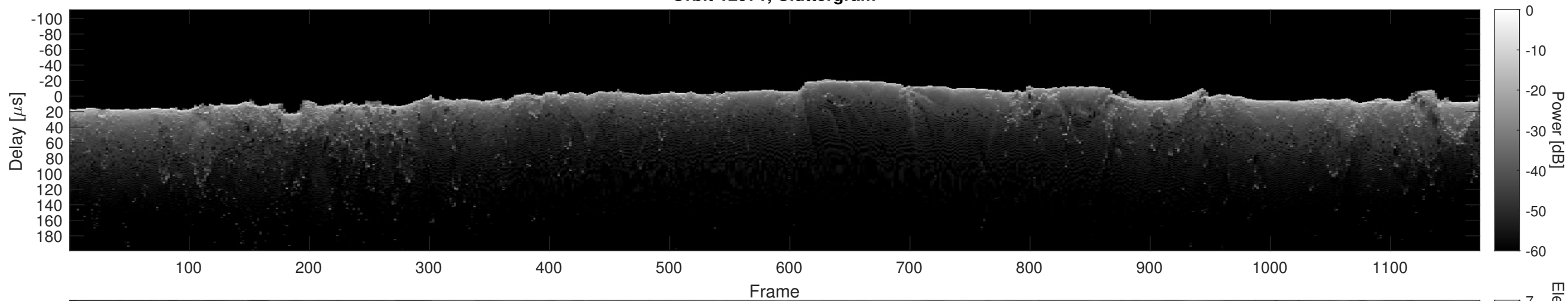
Orbit 12971, Cluttergram
