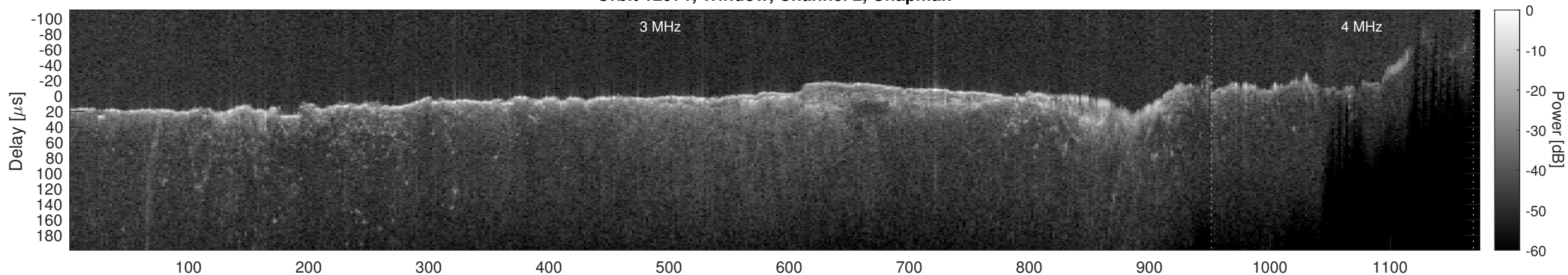
Orbit 12971, Window, Channel 2, Optimized
