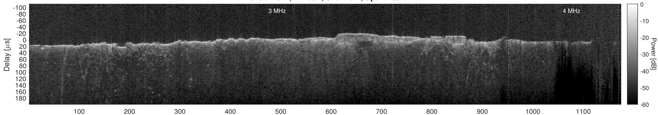
Orbit 12971, Cluttergram
