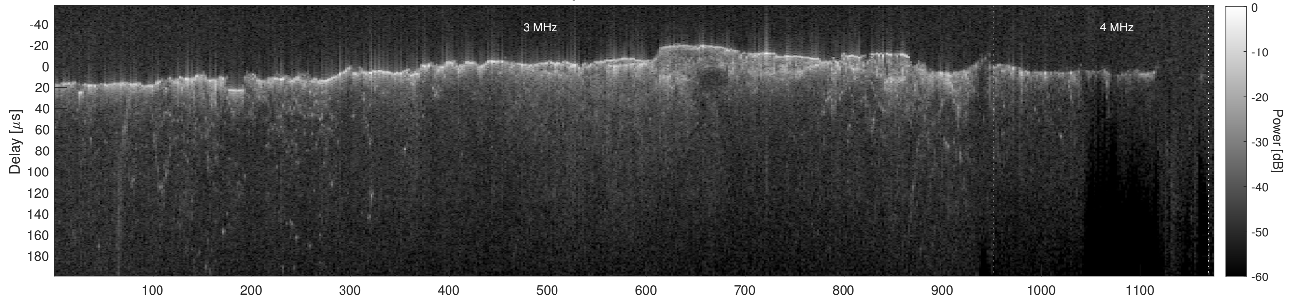
Orbit 12971, Cluttergram
