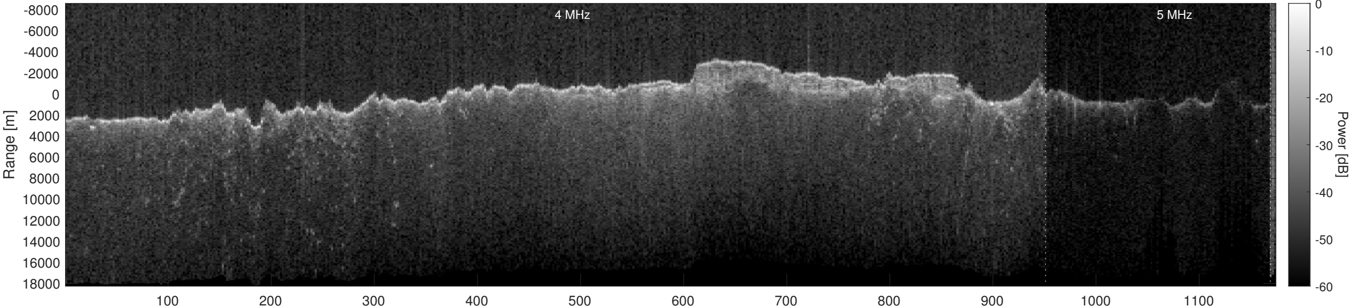
Orbit 12971, Optimized, Window, Depth-Corrected, Channel 2
