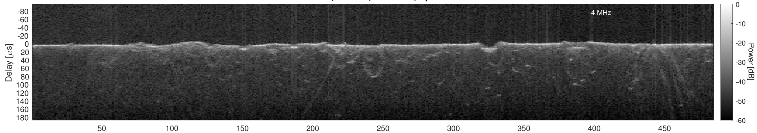
Orbit 12972, Cluttergram
