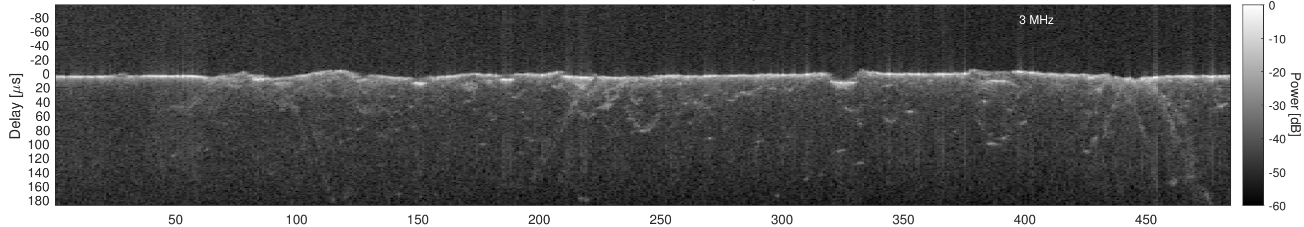
Orbit 12972, Window, Channel 2, Optimized
