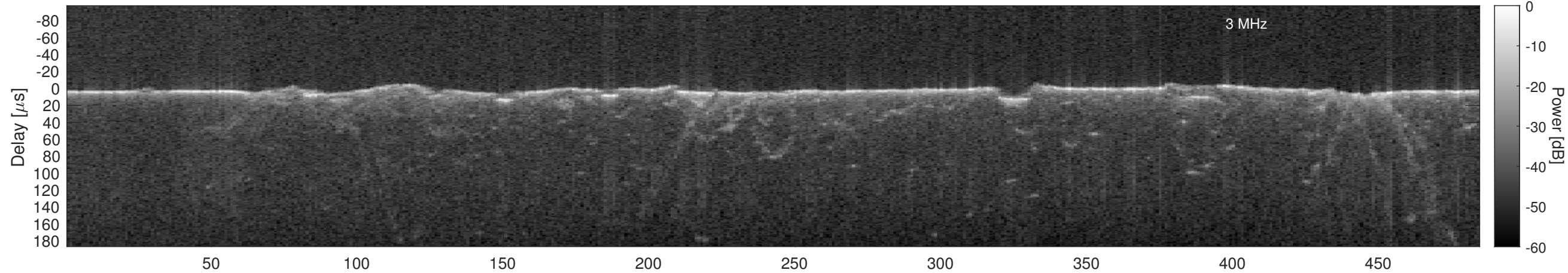
Orbit 12972, Window, Channel 2, Chapman
