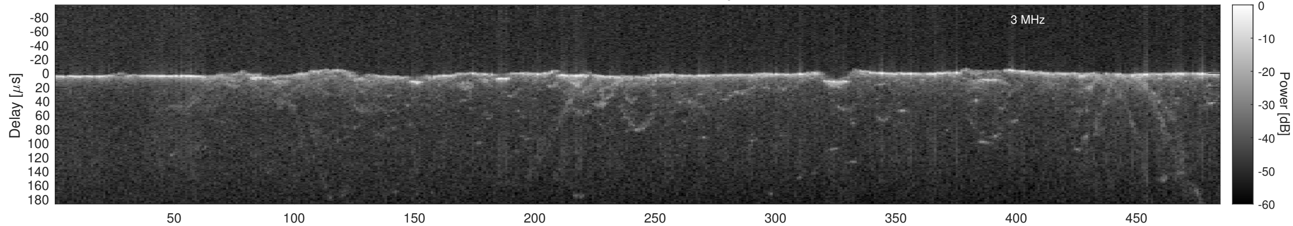
Orbit 12972, Cluttergram
