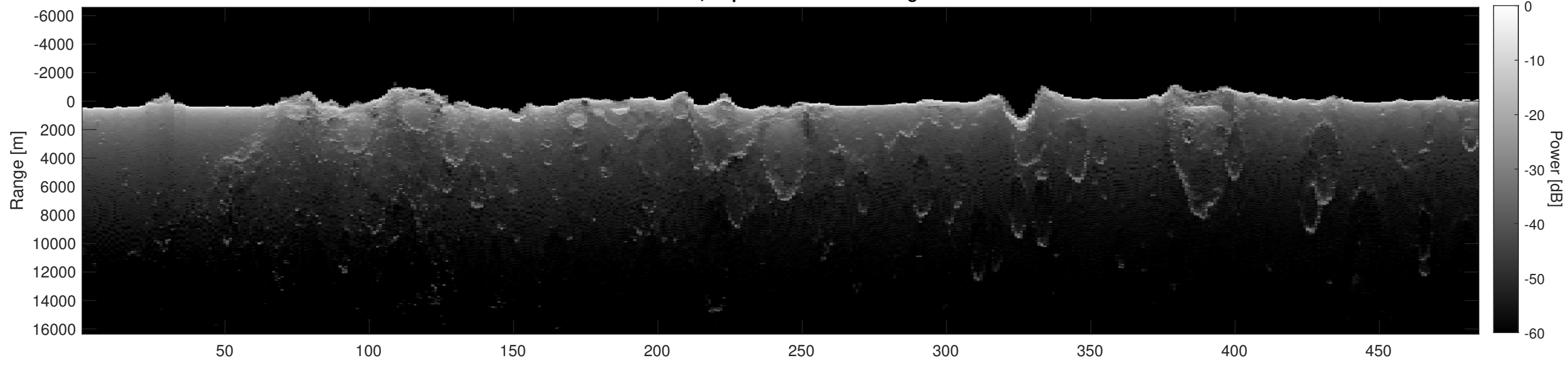
Orbit 12972, Depth-Corrected Cluttergram
