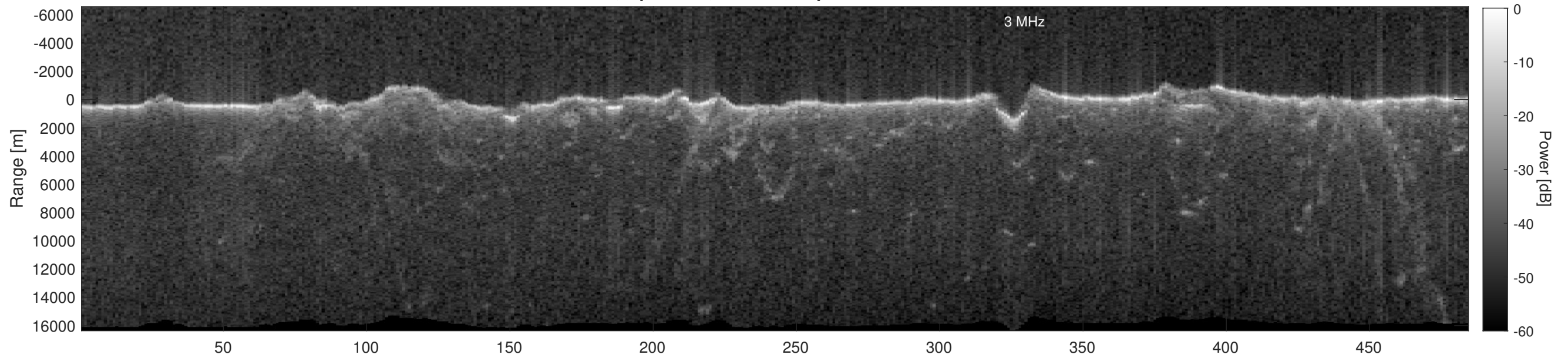
Orbit 12972, Depth-Corrected Cluttergram
