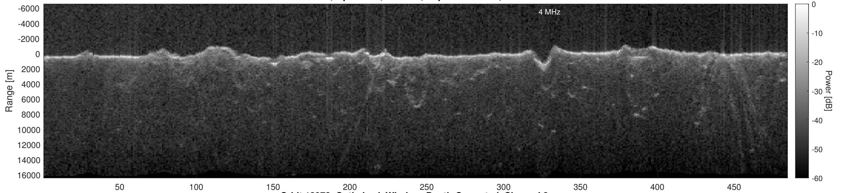
Orbit 12972, Optimized, Window, Depth-Corrected, Channel 2
