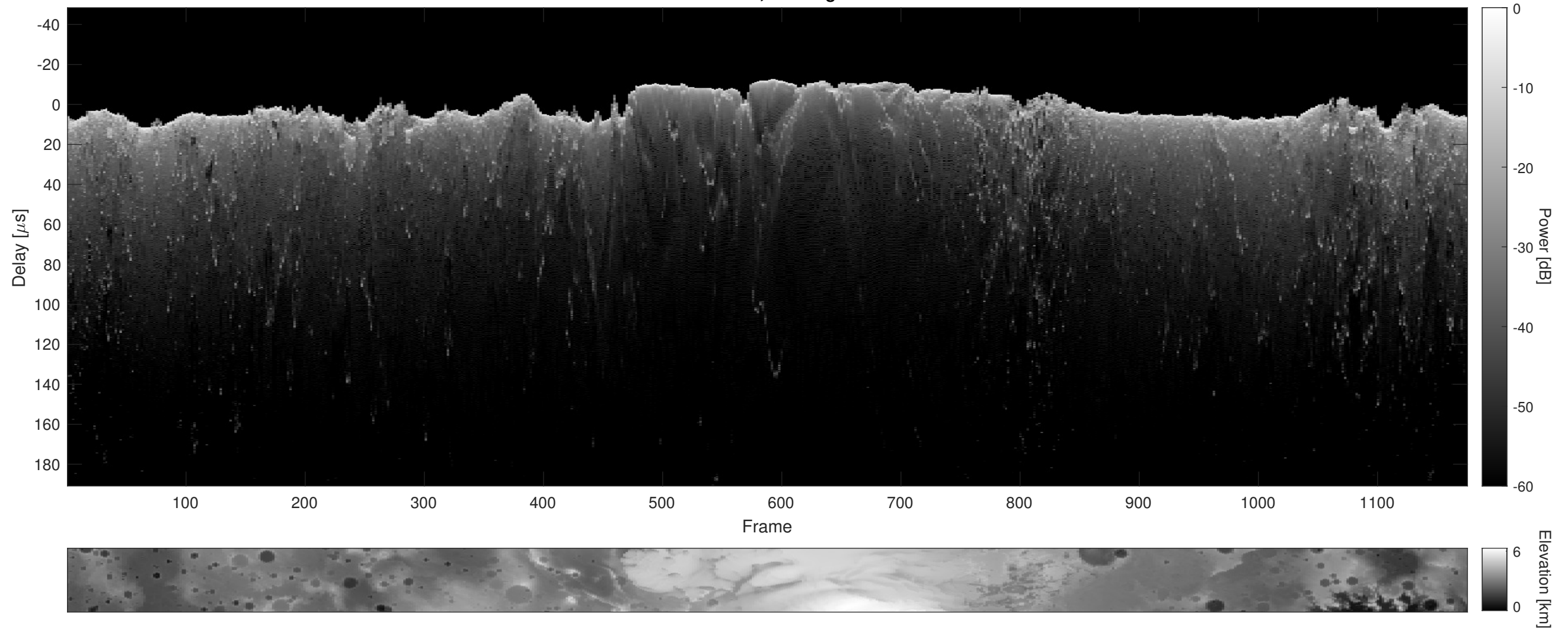
Orbit 12973, Cluttergram
