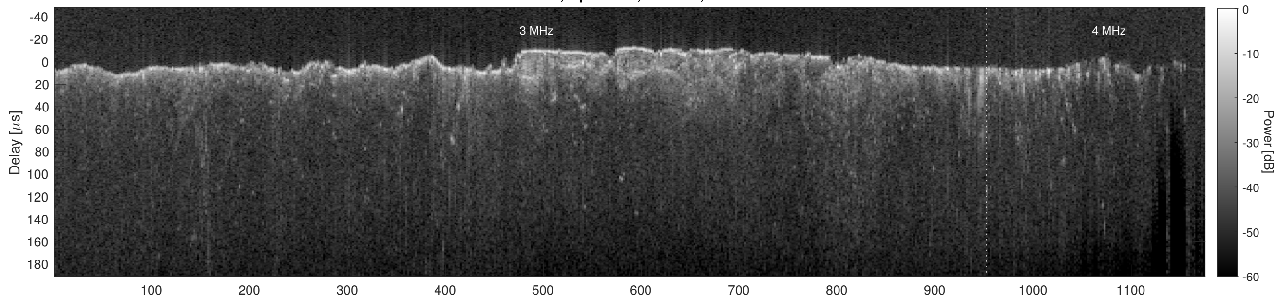
Orbit 12973, Cluttergram
