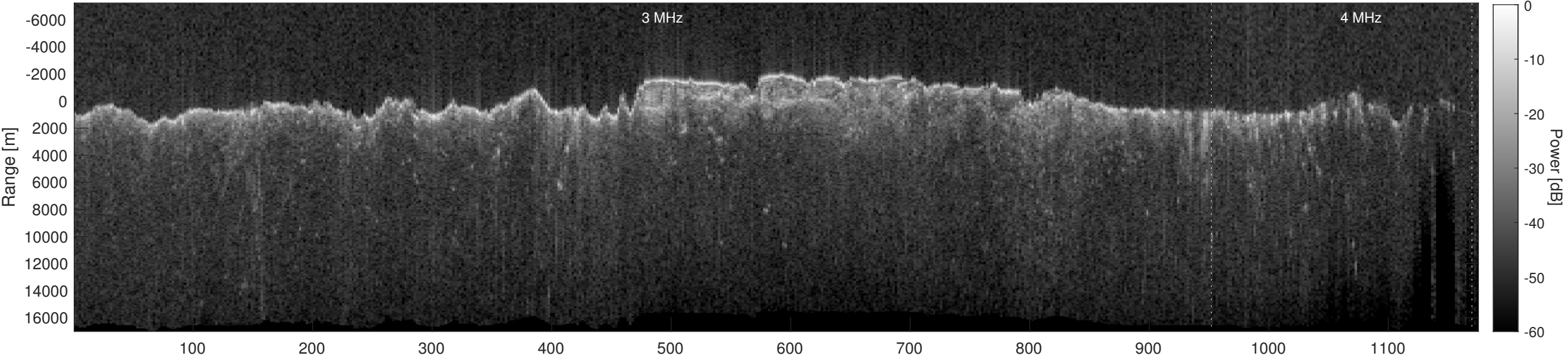
Orbit 12973, Depth-Corrected Cluttergram
