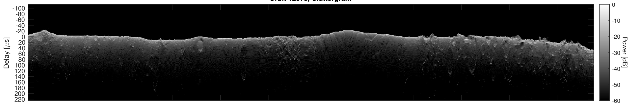
Orbit 12975, Cluttergram
