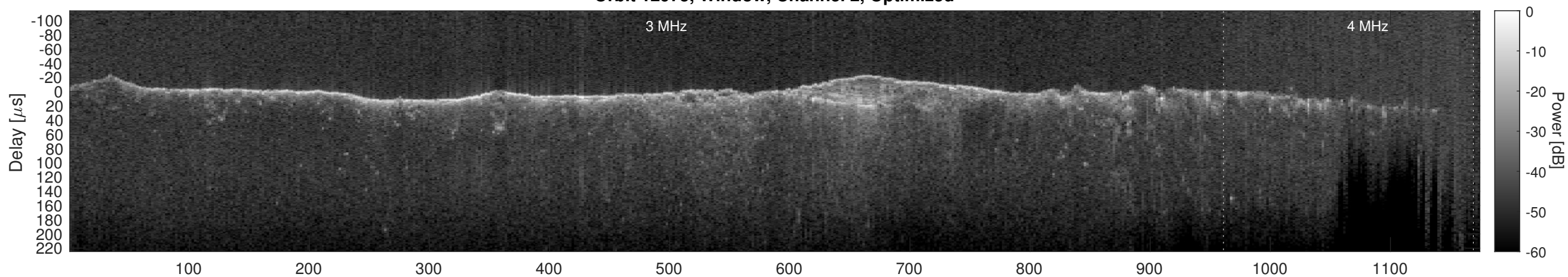
Orbit 12975, Cluttergram
