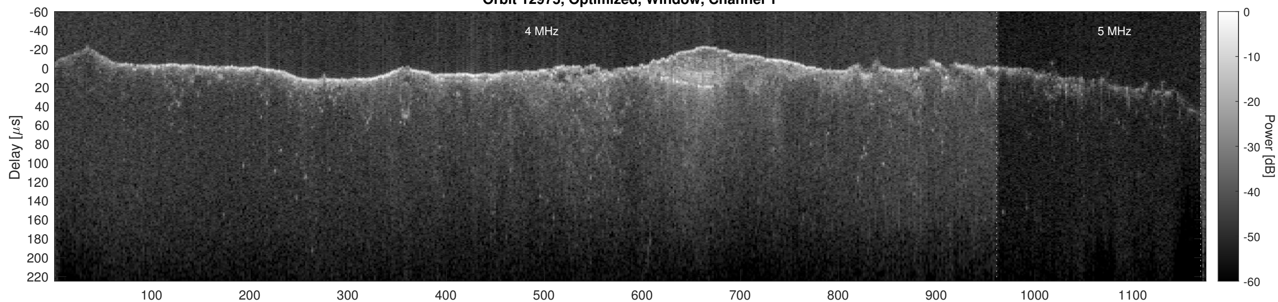
Orbit 12975, Optimized, Window, Channel 2
