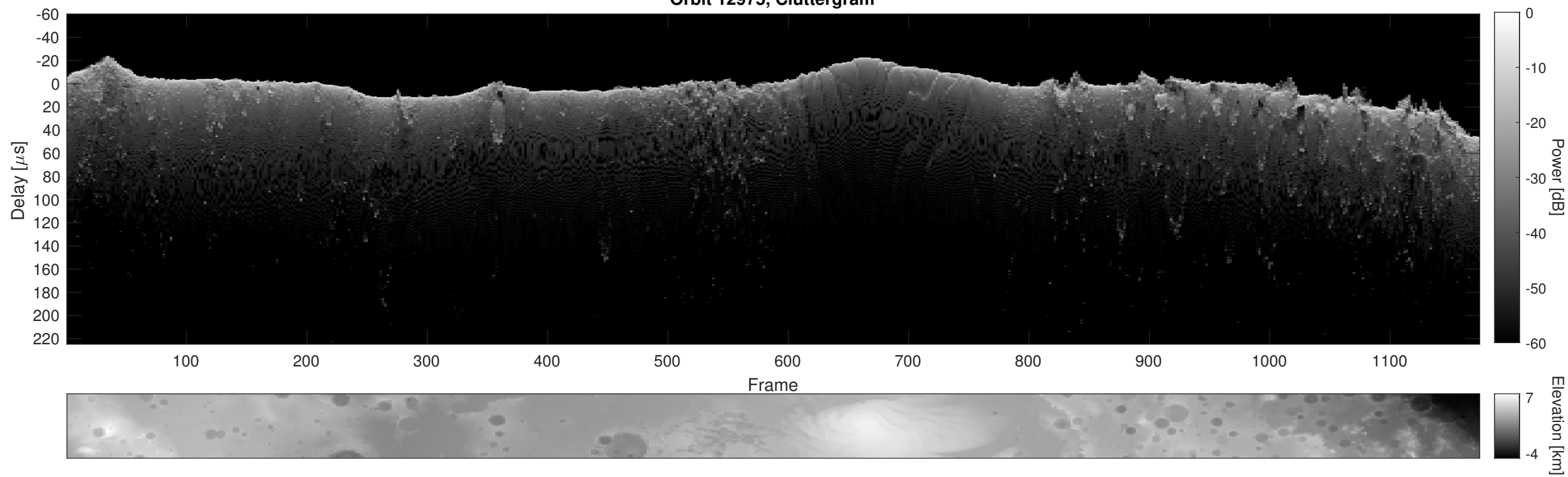
Orbit 12975, Cluttergram
