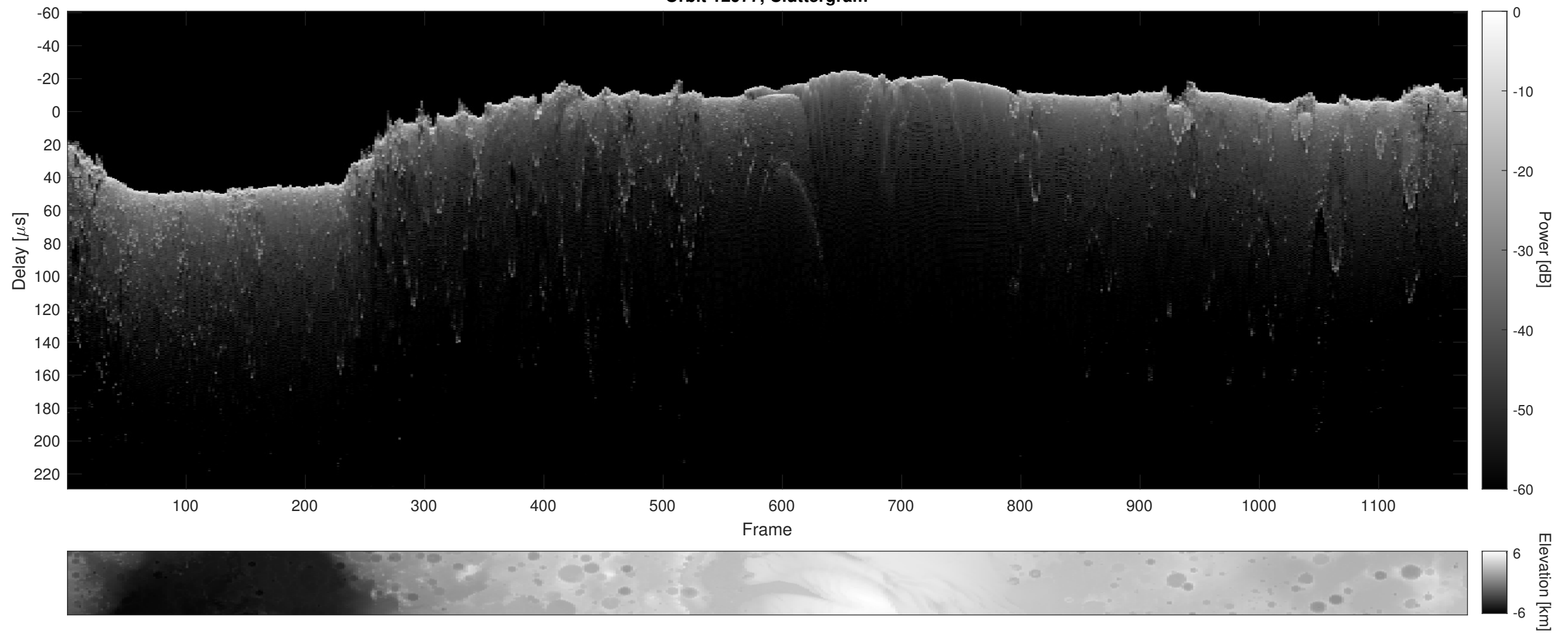
Orbit 12977, Cluttergram
