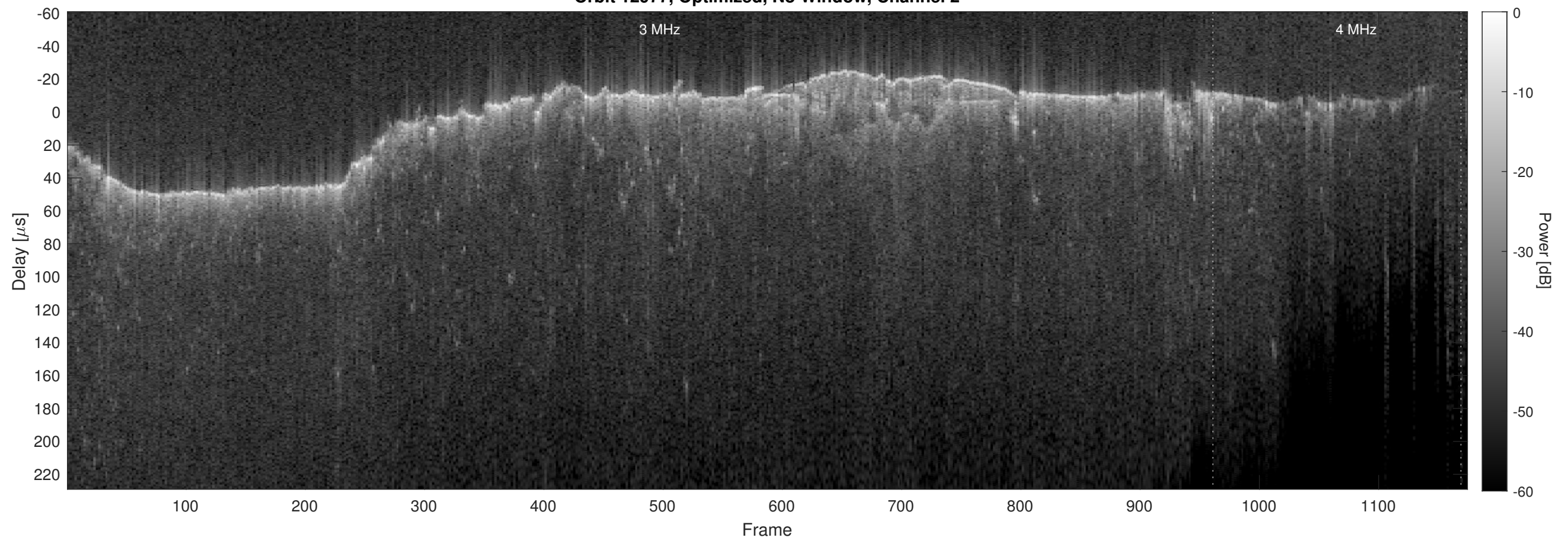
Orbit 12977, Optimized, No Window, Channel 2
