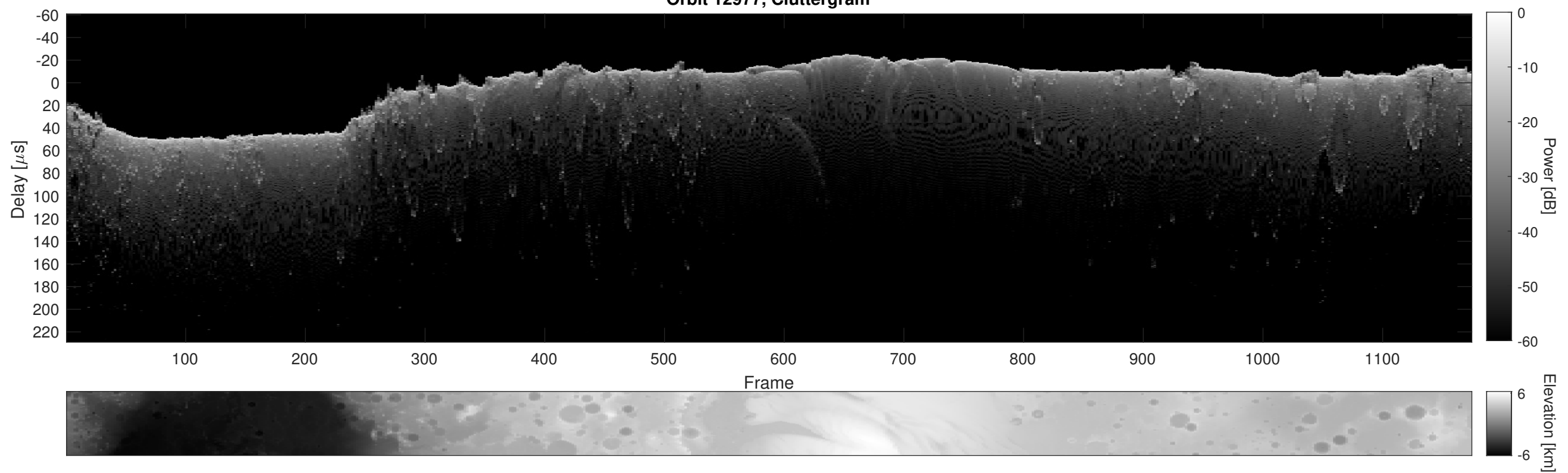
Orbit 12977, Cluttergram
