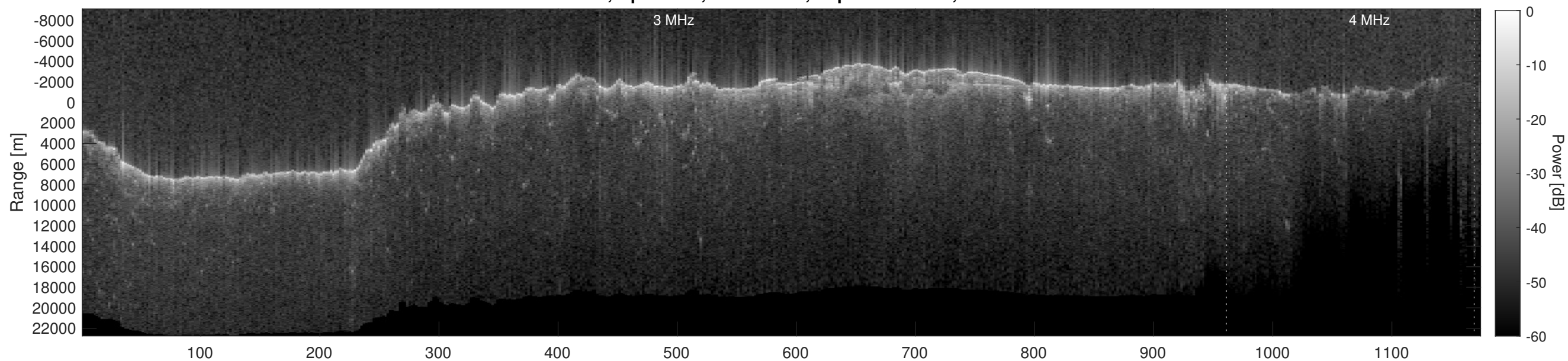
Orbit 12977, Depth-Corrected Cluttergram
