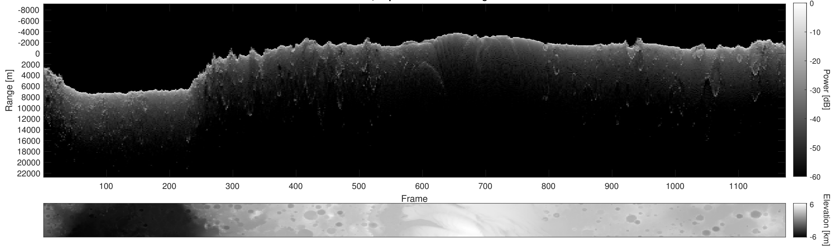
Orbit 12977, Depth-Corrected Cluttergram
