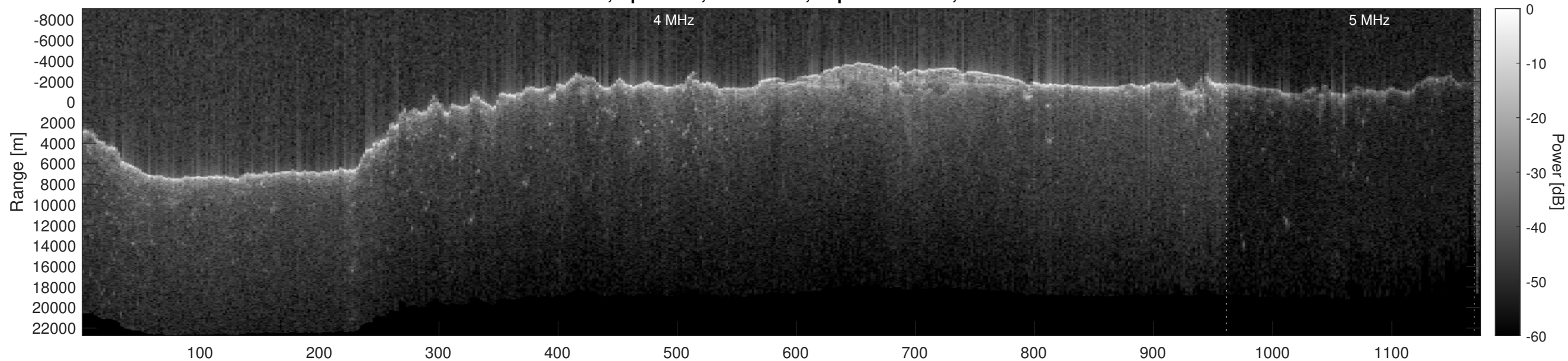
Orbit 12977, Optimized, No Window, Depth-Corrected, Channel 2
