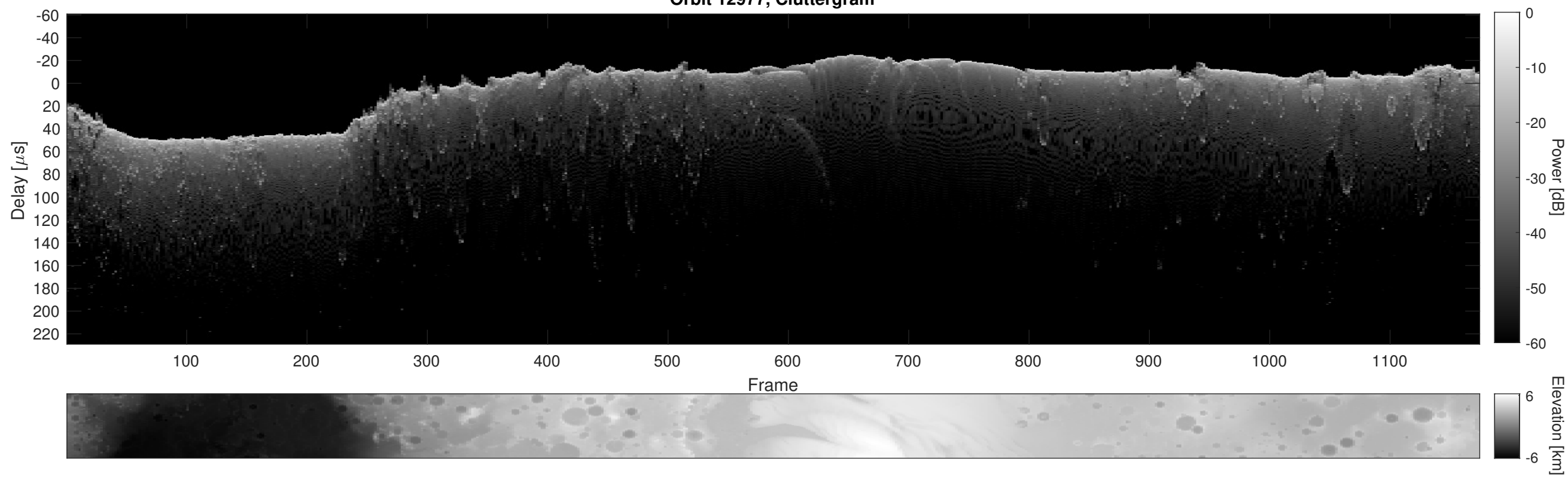
Orbit 12977, Cluttergram
