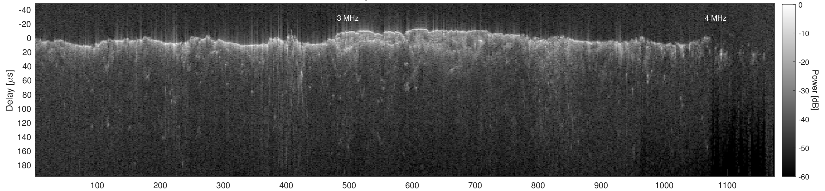
Orbit 12980, Cluttergram
