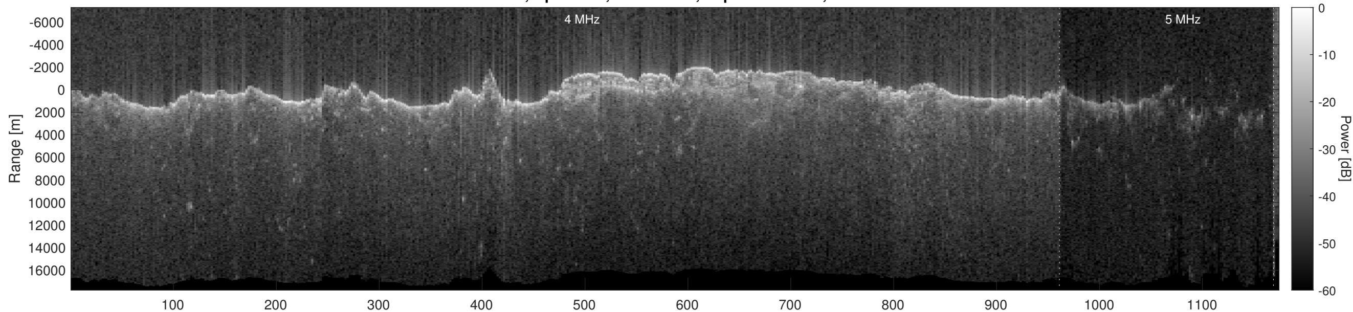
Orbit 12980, Optimized, No Window, Depth-Corrected, Channel 2
