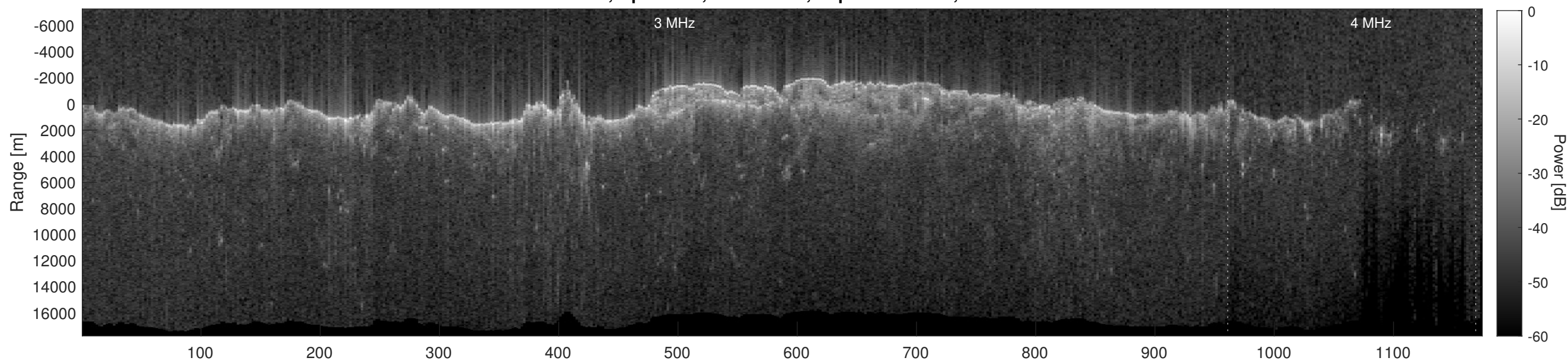
Orbit 12980, Depth-Corrected Cluttergram
