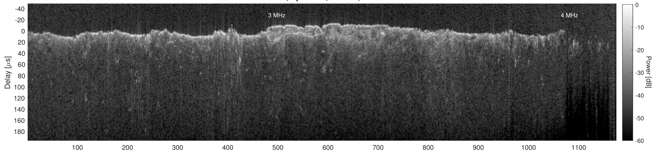
Orbit 12980, Cluttergram
