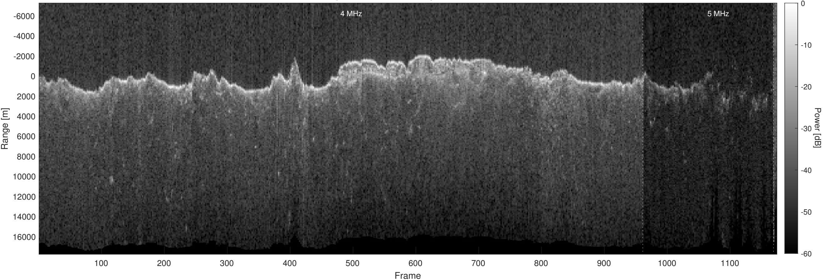
Orbit 12980, Optimized, Window, Depth-Corrected, Channel 2
