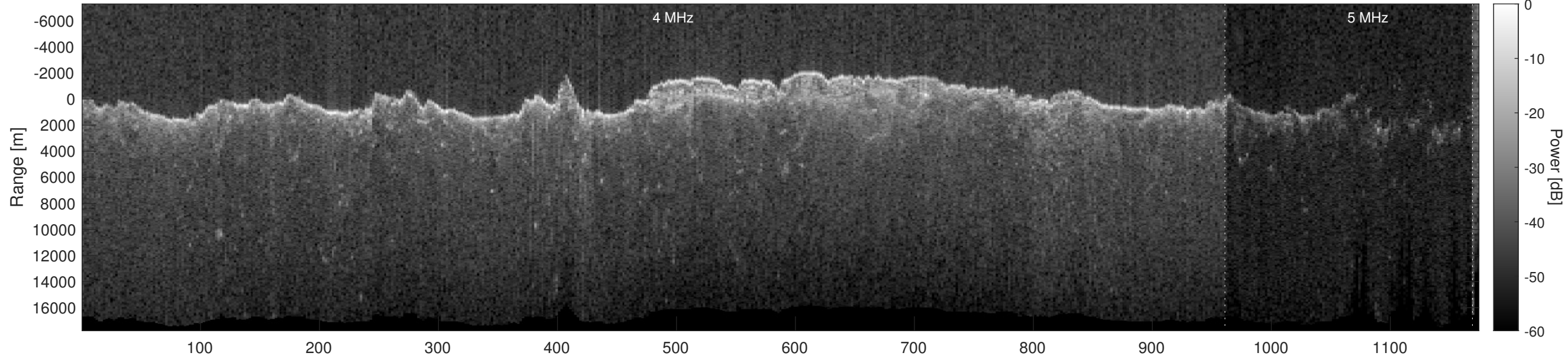
Orbit 12980, Optimized, Window, Depth-Corrected, Channel 2
