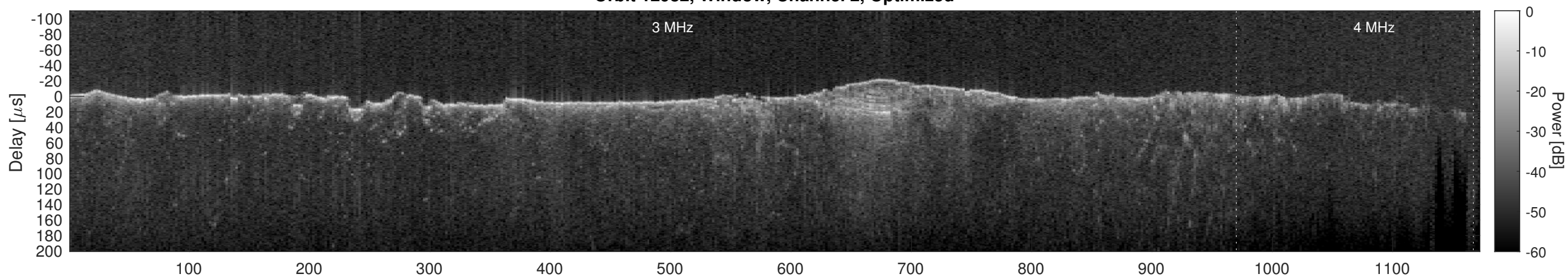
Orbit 12982, Cluttergram
